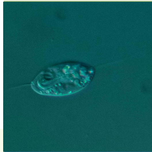
FLAGELLAT 4 – 30 \mu\text{m}
